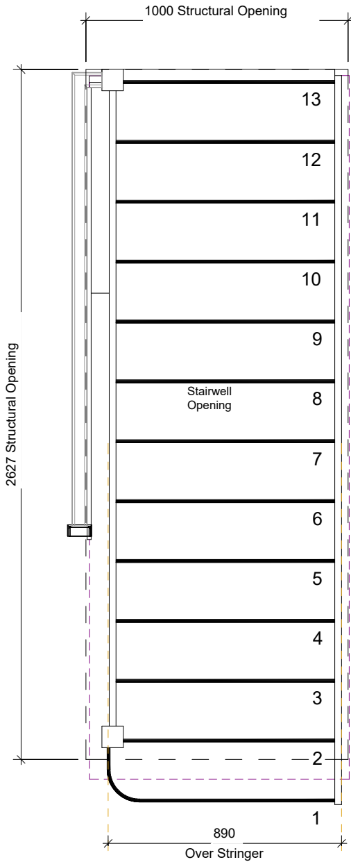
1 Staircase - Plan 1 : 20
